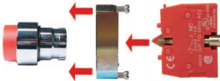
Metal Chrome Bezel Steel Block Holder Included with operators Bolt - On Contact Block
