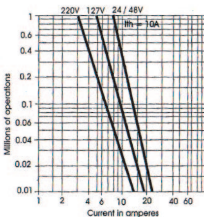
DC Ratings, UL Type Q600 Inductive and resistive Amps
