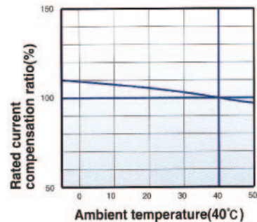
Ambient Compensation Ration Chart for 300-800Amp
