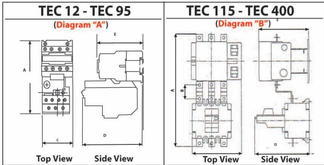
Dimension Details For TEC12-TEC95 / Direct Mount
