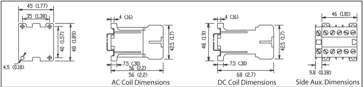
Type LS05, SH05, and HS05 (frame size I, Lateral) with screw terminals.
