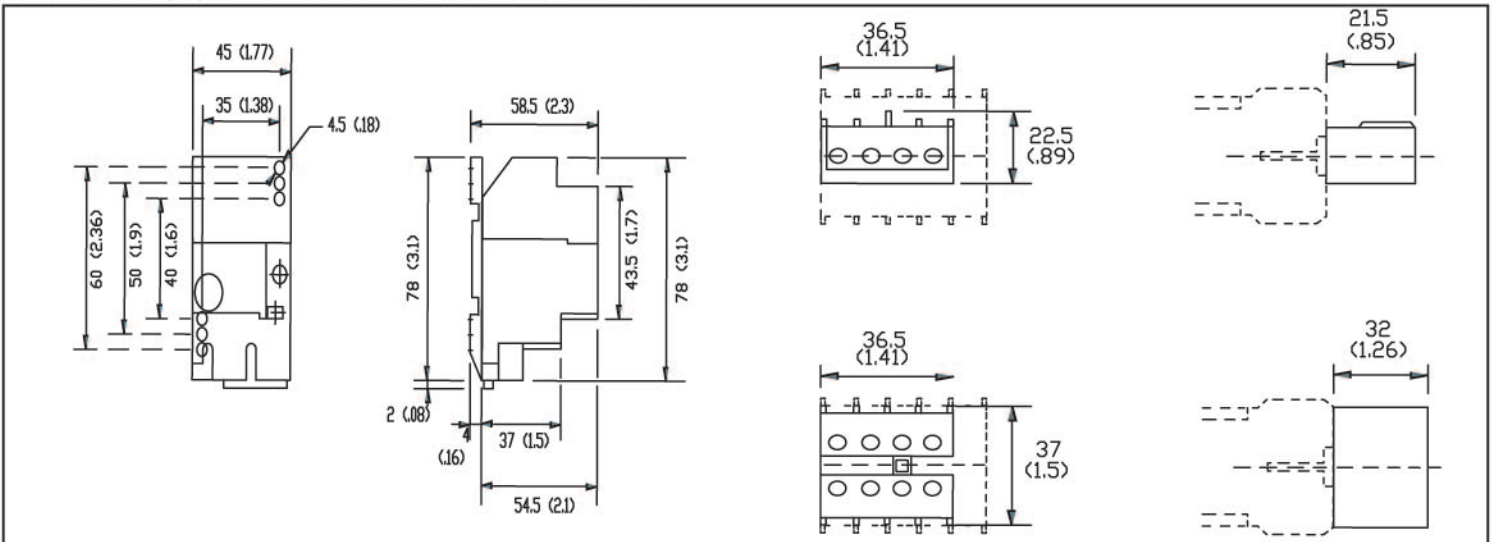
Terminal block & snap-on adaptor for type B05, independent mounting Type HS05 (frame size II & IV frontal mounting) with screw terminals
