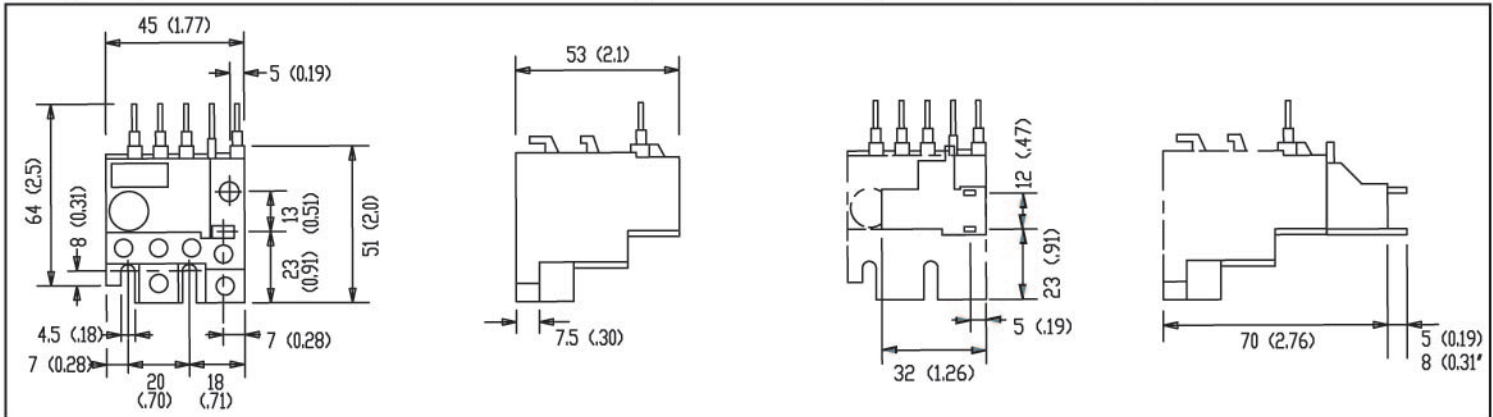
Overload relay type B05 for mounting on contactors
